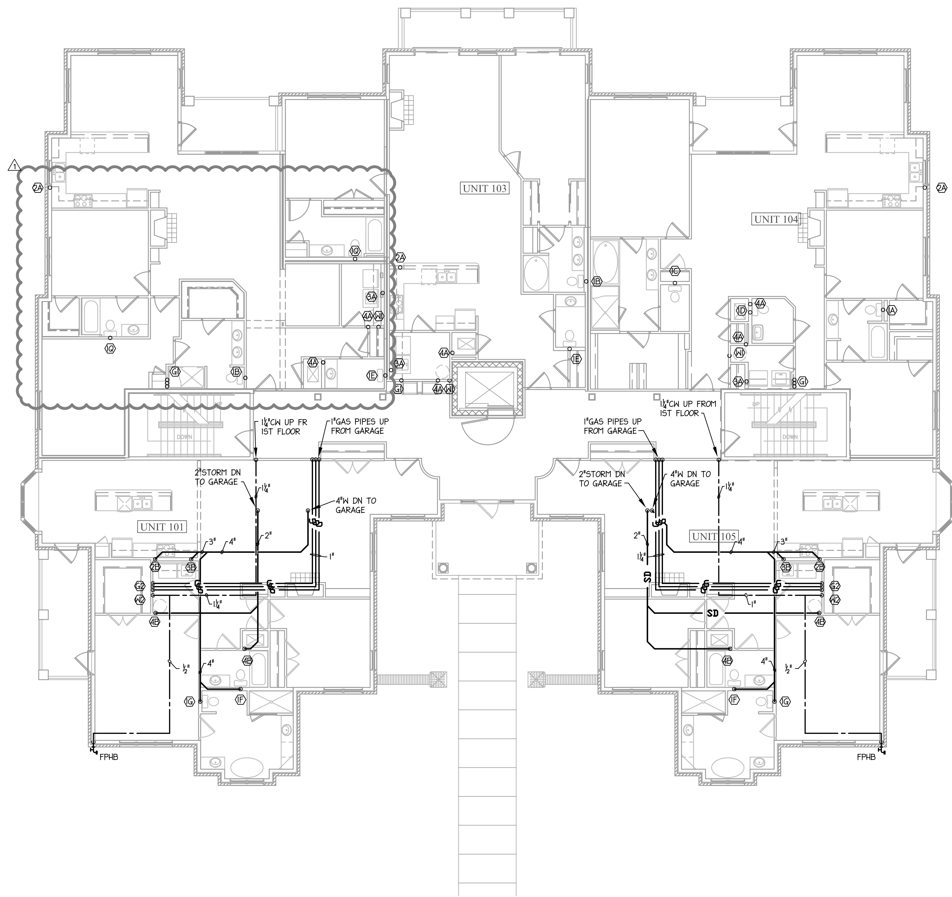
1 RESIDENTIAL LEVEL 2 1/8" = 1'-0"
