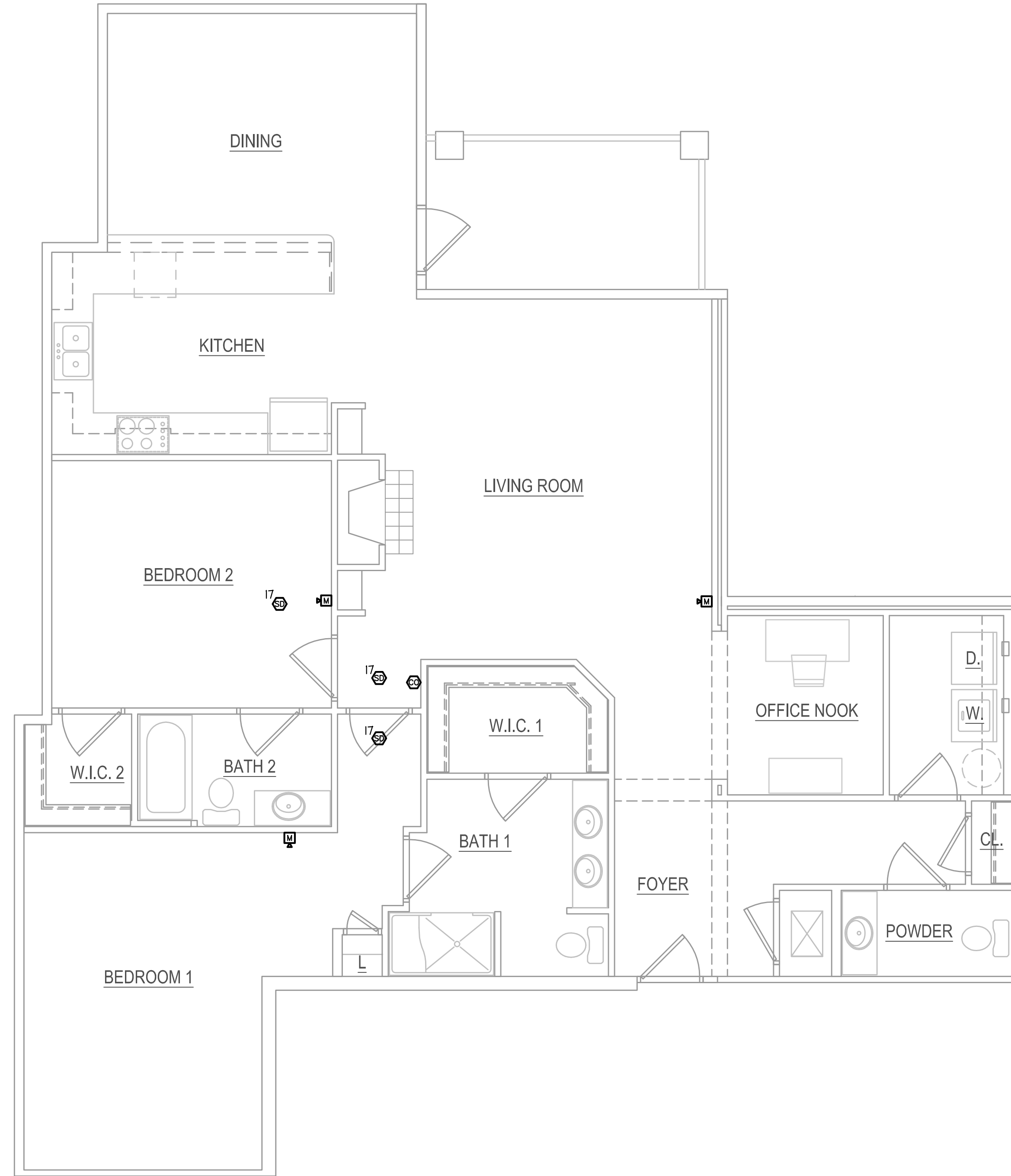
1 UNIT 4 1/4" = 1'-0"
