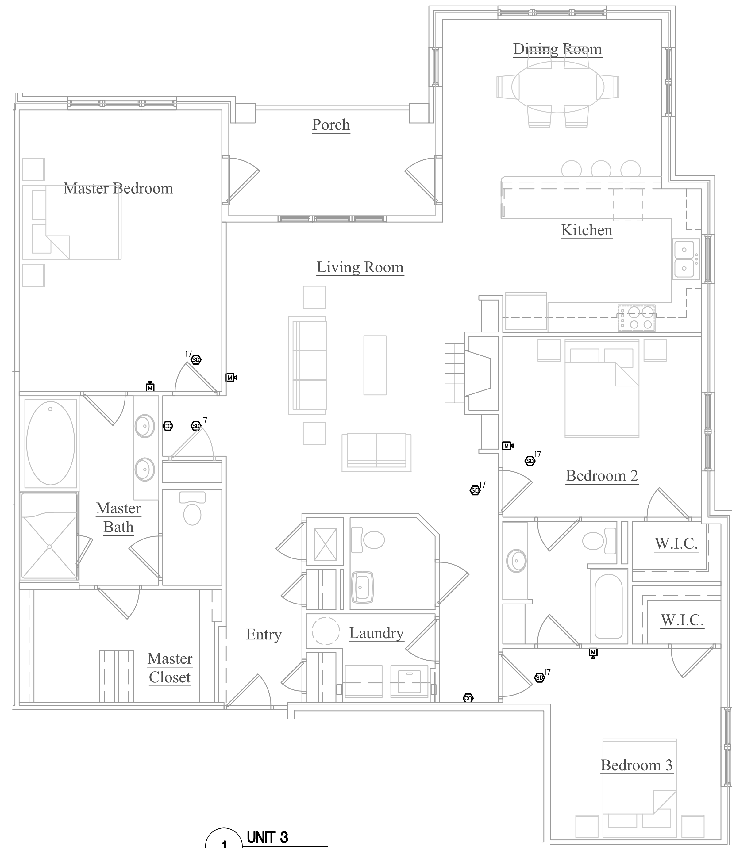
1 UNIT 3 1/4" = 1'-0"
