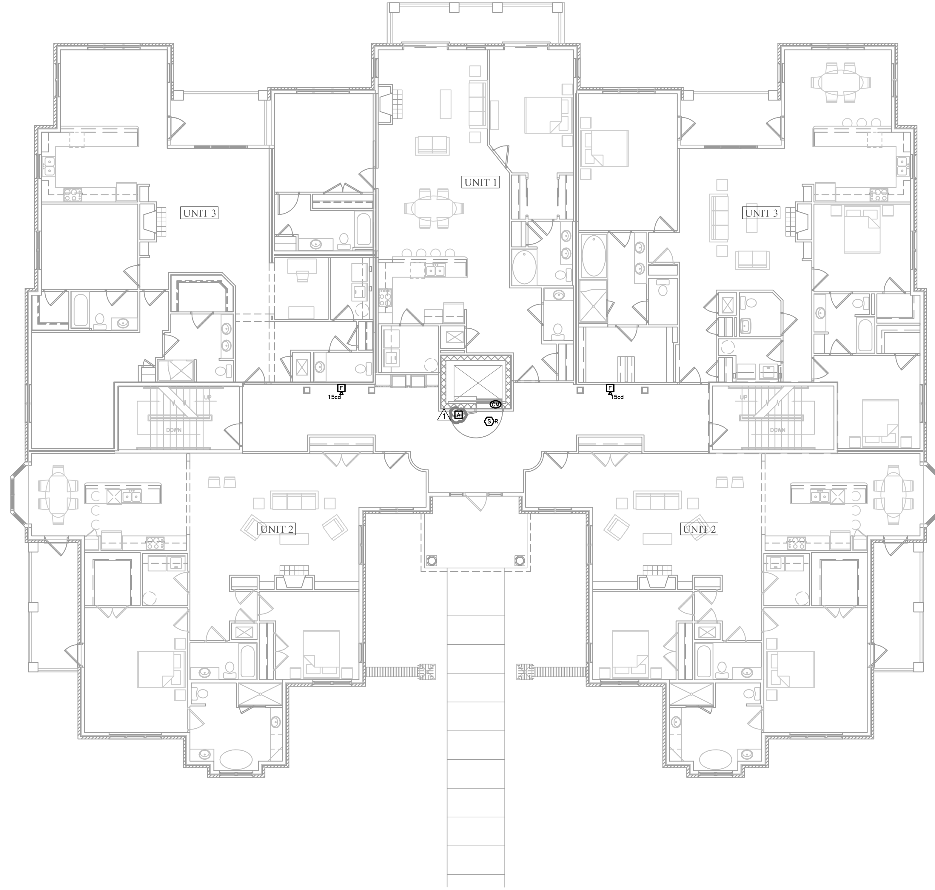
1 RESIDENTIAL LEVEL 2 1/8" = 1'-0"
